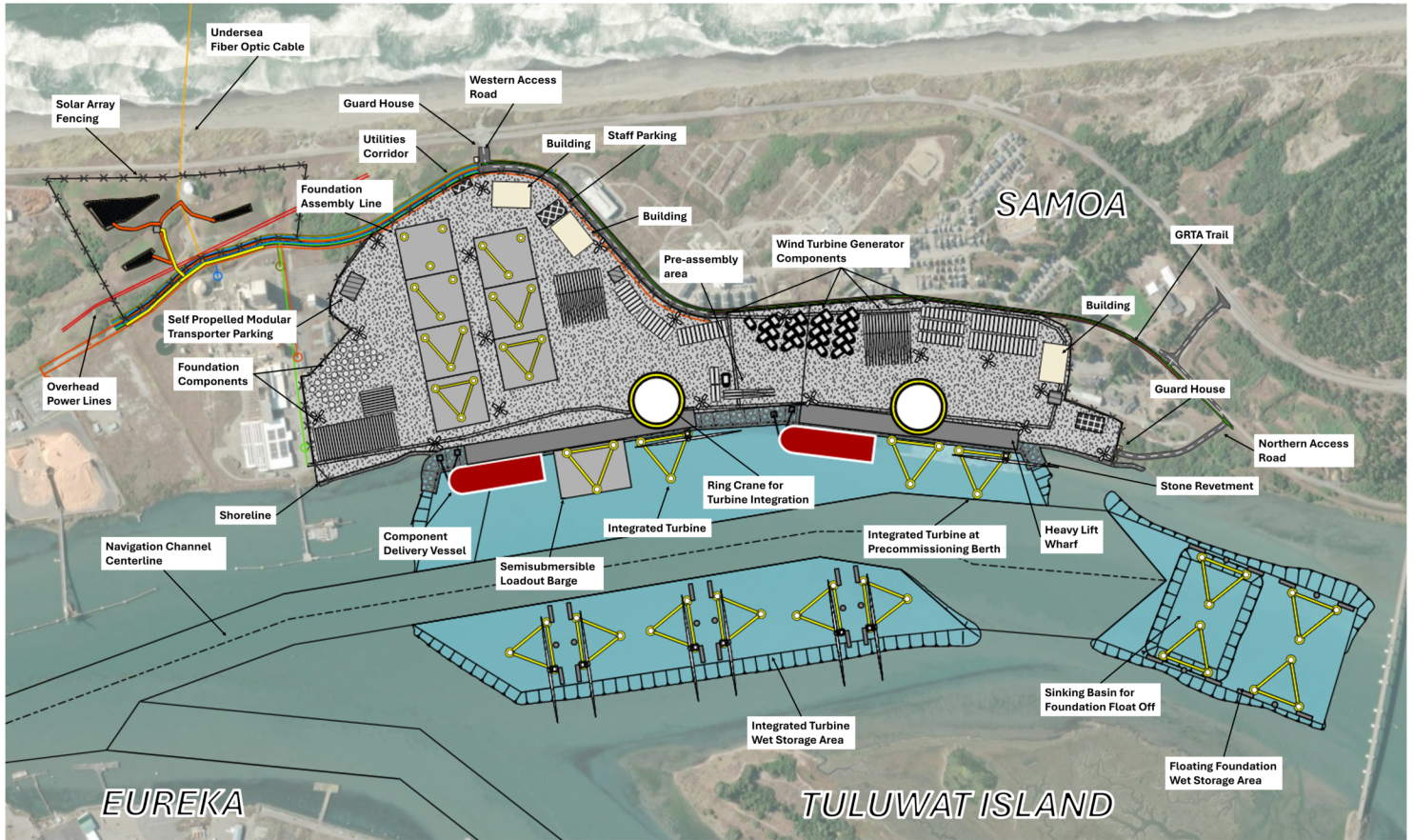
HUMBOLDT HEAVY LIFT MARINE TERMINAL SITE LAYOUT
