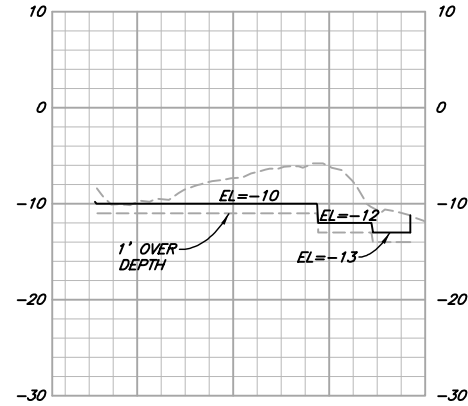
SECTION D SCALE: 1"=100' H 1"=10' V
