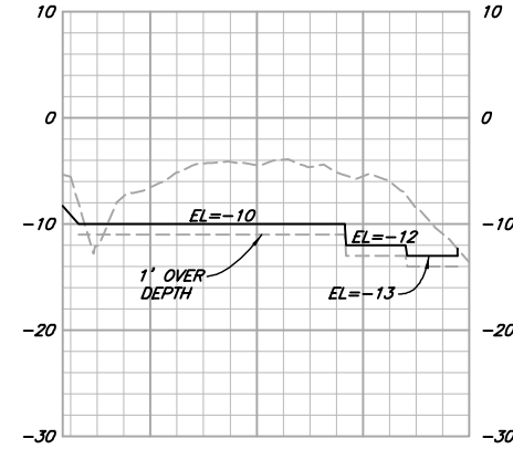
SECTION G SCALE: 1"=100' H 1"=10' V
