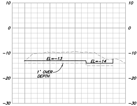
SECTION A SCALE: 1"=100' H 1"=10' V
