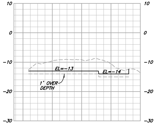
SECTION B SCALE: 1"=100' H 1"=10' V
