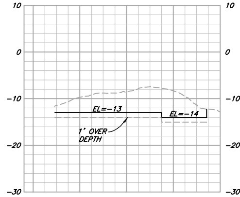
SECTION C SCALE: 1"=100' H 1"=10' V
