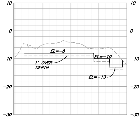
SECTION H SCALE: 1"=100' H 1"=10' V
