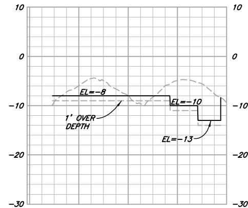
SECTION J SCALE: 1"=100' H 1"=10' V
