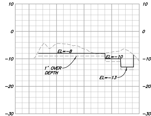
SECTION I SCALE: 1"=100' H 1"=10' V
